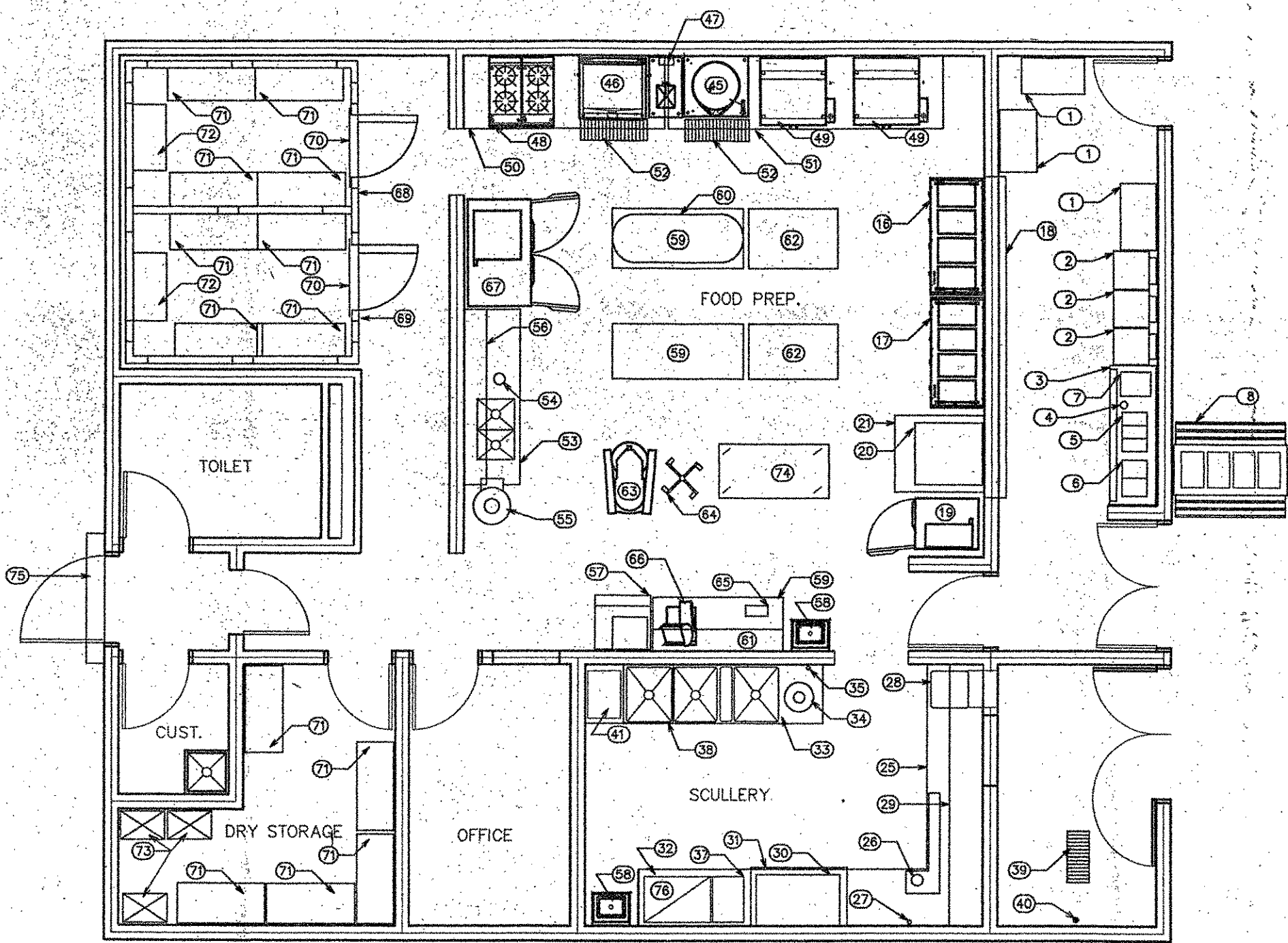
KITCHEN PLAN 1/4"=1'-0"
